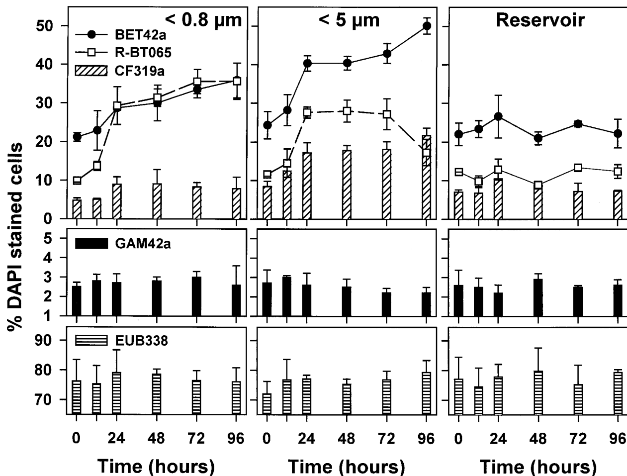
FIG. 4. Time course changes in the phylogenetic composition of the bacterioplankton community in size fractionation treatments ( <0.8 and <5 \mu\text{m} ) exposed in dialysis bags compared to unfiltered reservoir water during the experiment. Shown are proportions of beta proteobacteria and cells detected by probe R-BT065 (top), gamma proteobacteria (middle), CF group (CF319a, top), and total FISH detection rates by the general bacterial probe EUB338 (bottom). Values are means for three replicate treatments, and vertical bars show SDs.
